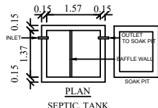
SEPTIC TANK
