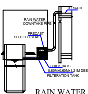
RAIN WATER
