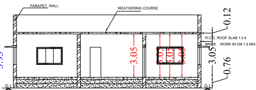
Section on-"AA"
