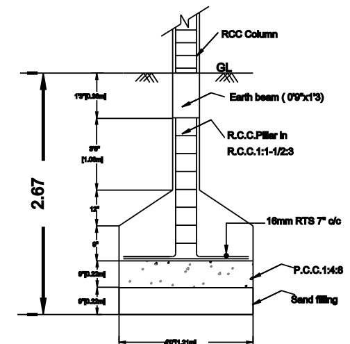
FOUNDATION DETAILS
