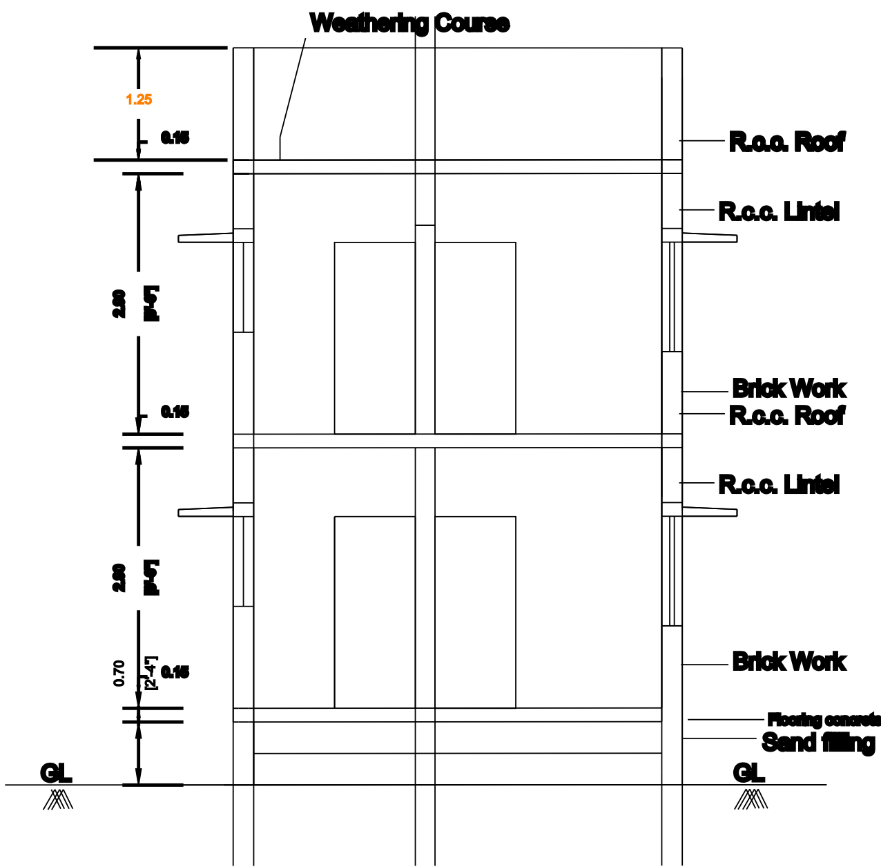
SECTION- BB
