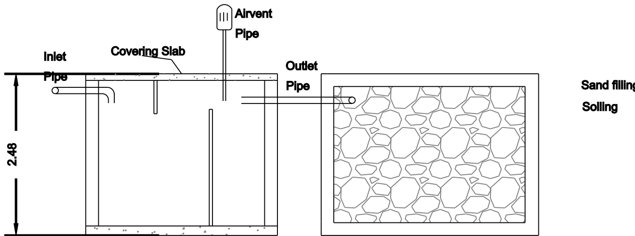
SECTION
