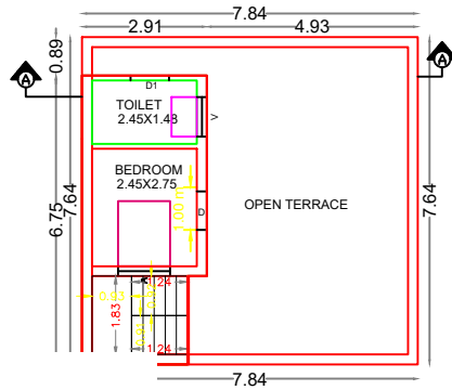
ED FIRST FLOOR PLAN
