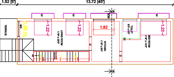
PRO.FIRST FLOOR PLAN
