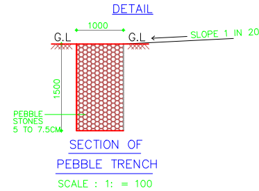
SECTION OF PEBBLE TRENCH
