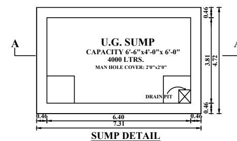
SUMP DETAIL
