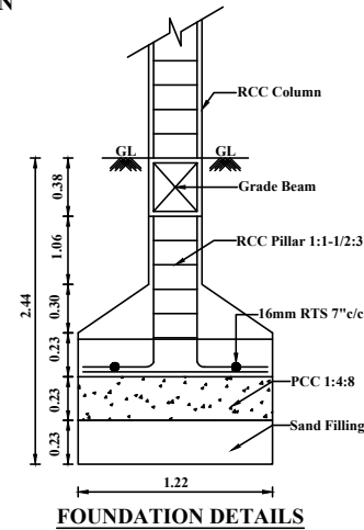
FOUNDATION DETAILS
