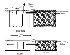
DETAILS OF SEPTIC TANK & DISPERSION TRENCH
