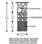
SECTION OF RAIN WATER COLLECTION PITS (NTS)
