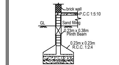
FOUNDATION DETAILS
