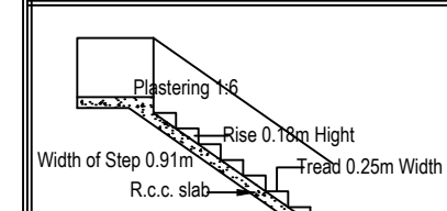
DETAILS OF STAIR CASE
