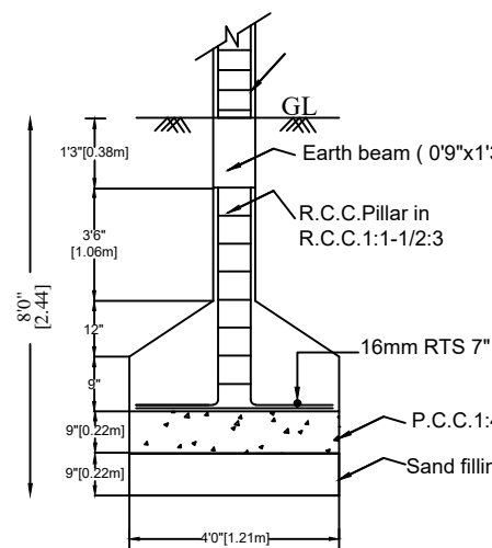
FOUNDATION DETAILS
