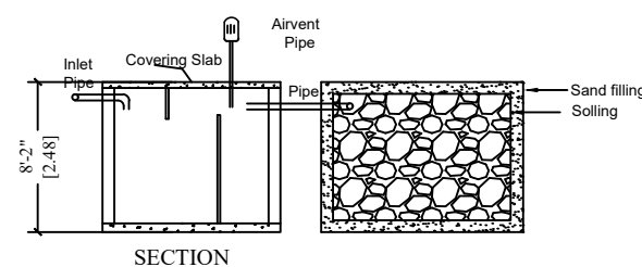
SECTION
