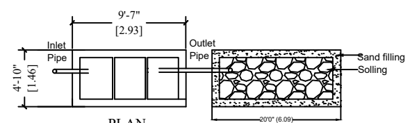
PLAN
