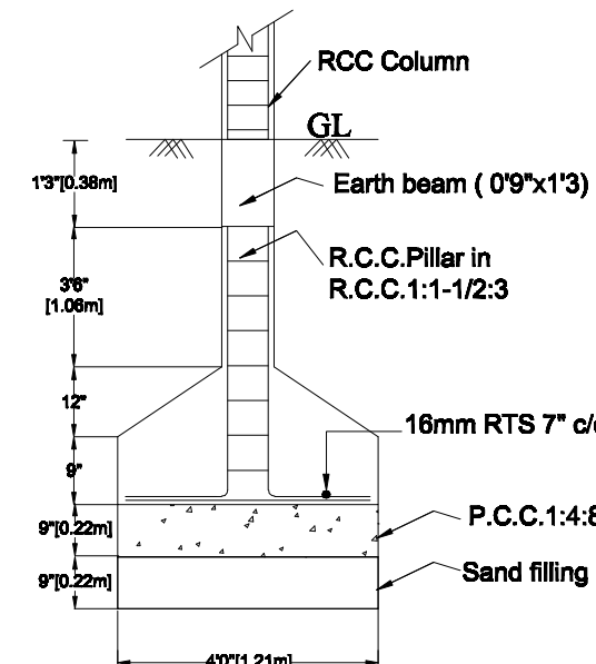
FOUNDATION DETAILS
