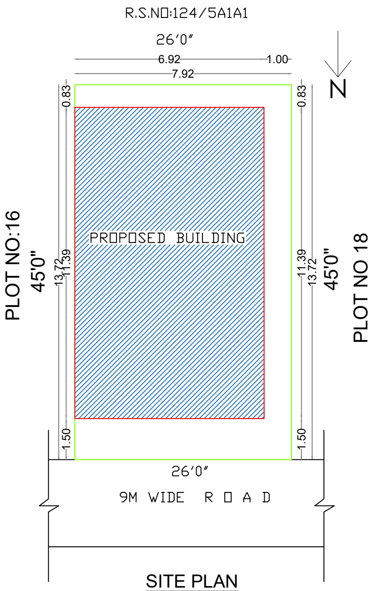
SITE PLAN
