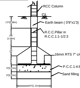
FOUNDATION DETAILS
