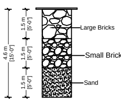
SECTION OF RAIN WATER COLLECTION PITS (N.T.S)
