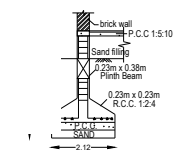
FOUNDATION DETAILS
