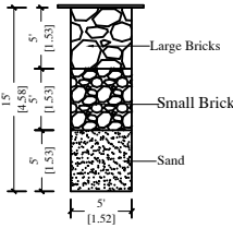
SECTION OF RAIN WATER COLLECTION PITS (NTS)
