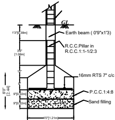
FOUNDATION DETAILS
