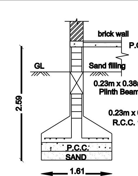
FOUNDATION DETAILS
