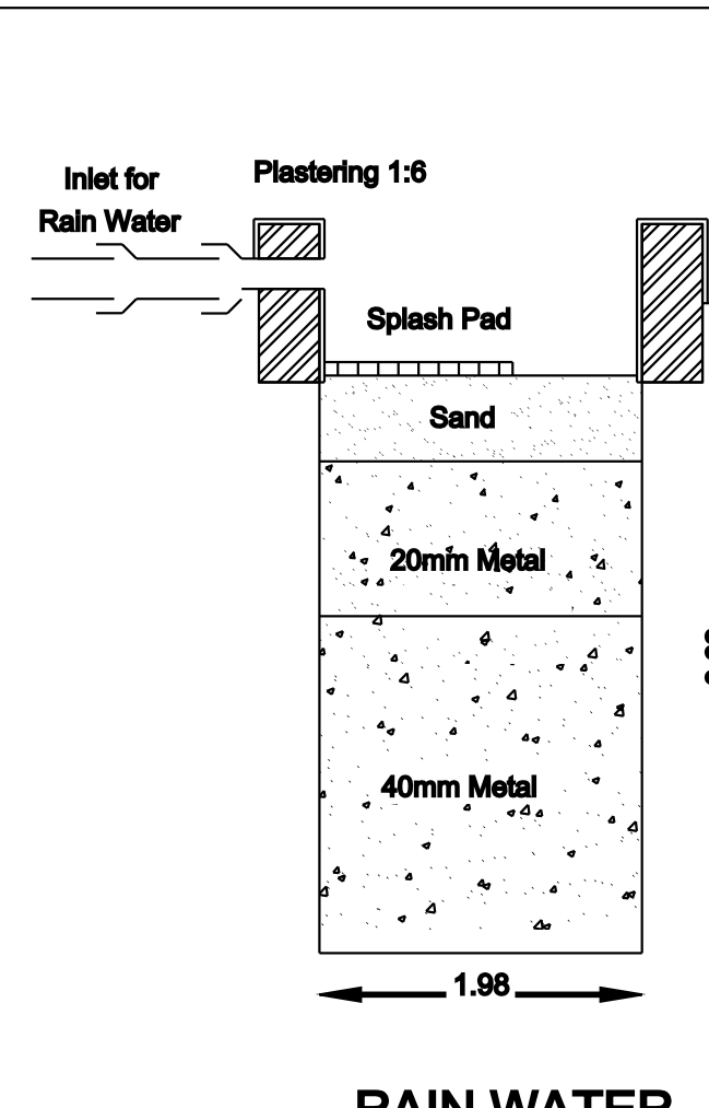
RAIN WATER
