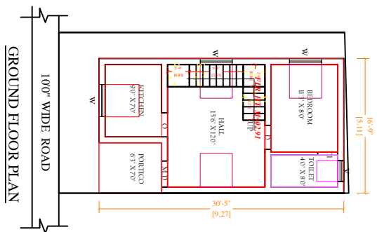
GROUND FLOOR AREA- 509 SFT
