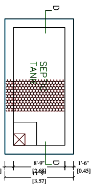
PLAN OF 10' x 20' SEPTIC TANK SCALE: 1" = 2'-0"
