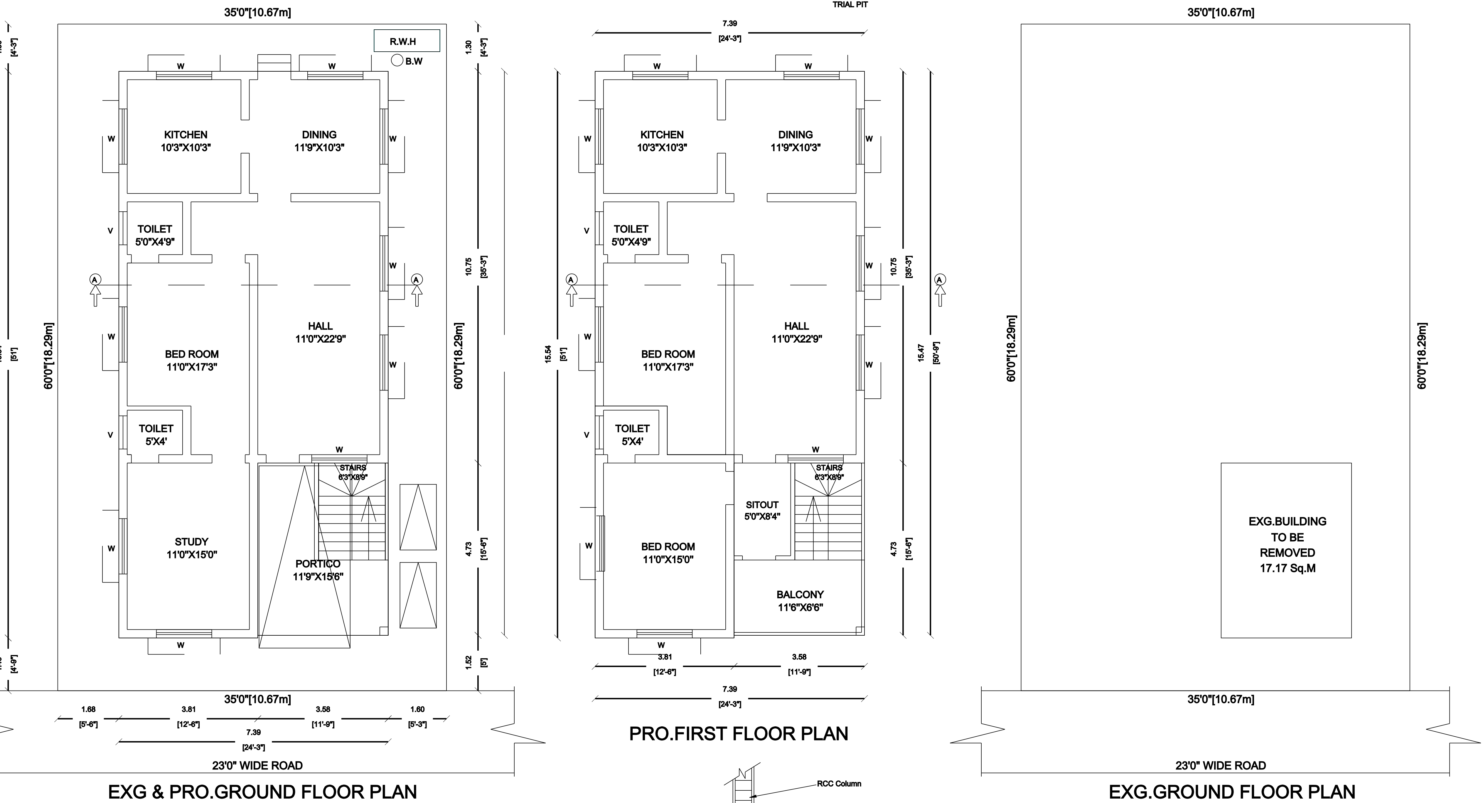
EXG.GROUND FLOOR PLAN
