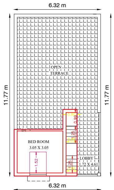
PRO.FIRST FLOOR PLAN
