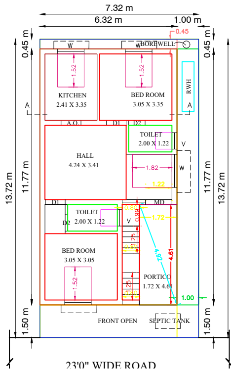
23'0" WIDE ROAD
