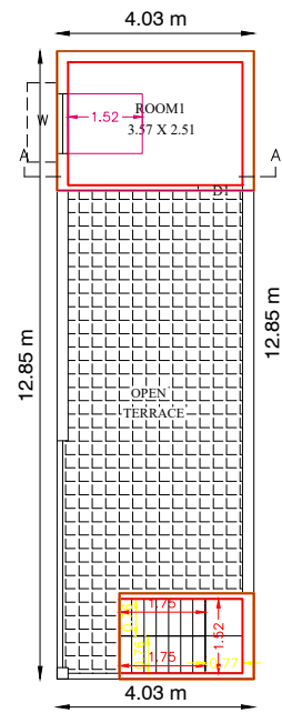
PRO.FIRST FLOOR PLAN
