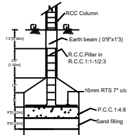
FOUNDATION DETAILS
