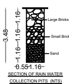
SECTION OF RAIN WATER COLLECTION PITS (NTS)
