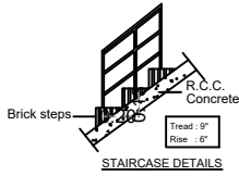
STAIRCASE DETAILS
