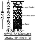
SECTION OF RAIN WATER COLLECTION PITS. (NTS)
