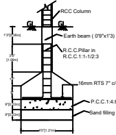
FOUNDATION DETAILS
