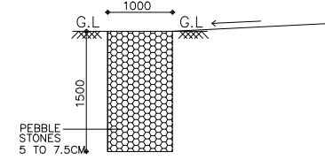
SECTION OF PEBBLE TRENCH
