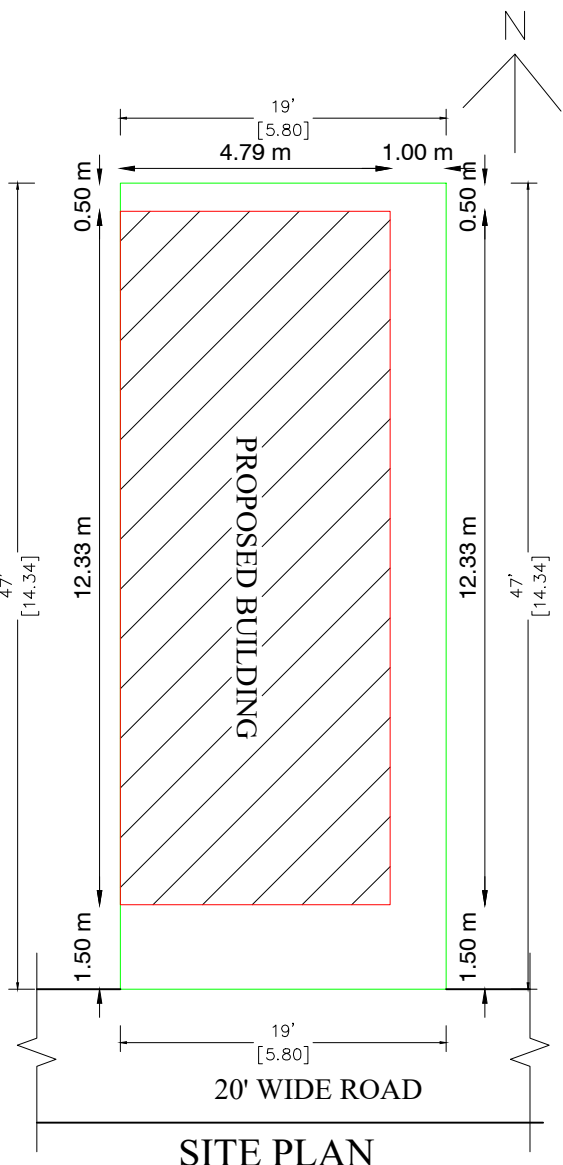
SITE PLAN
