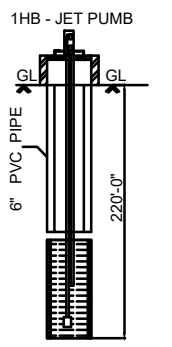
Bore Well Details
