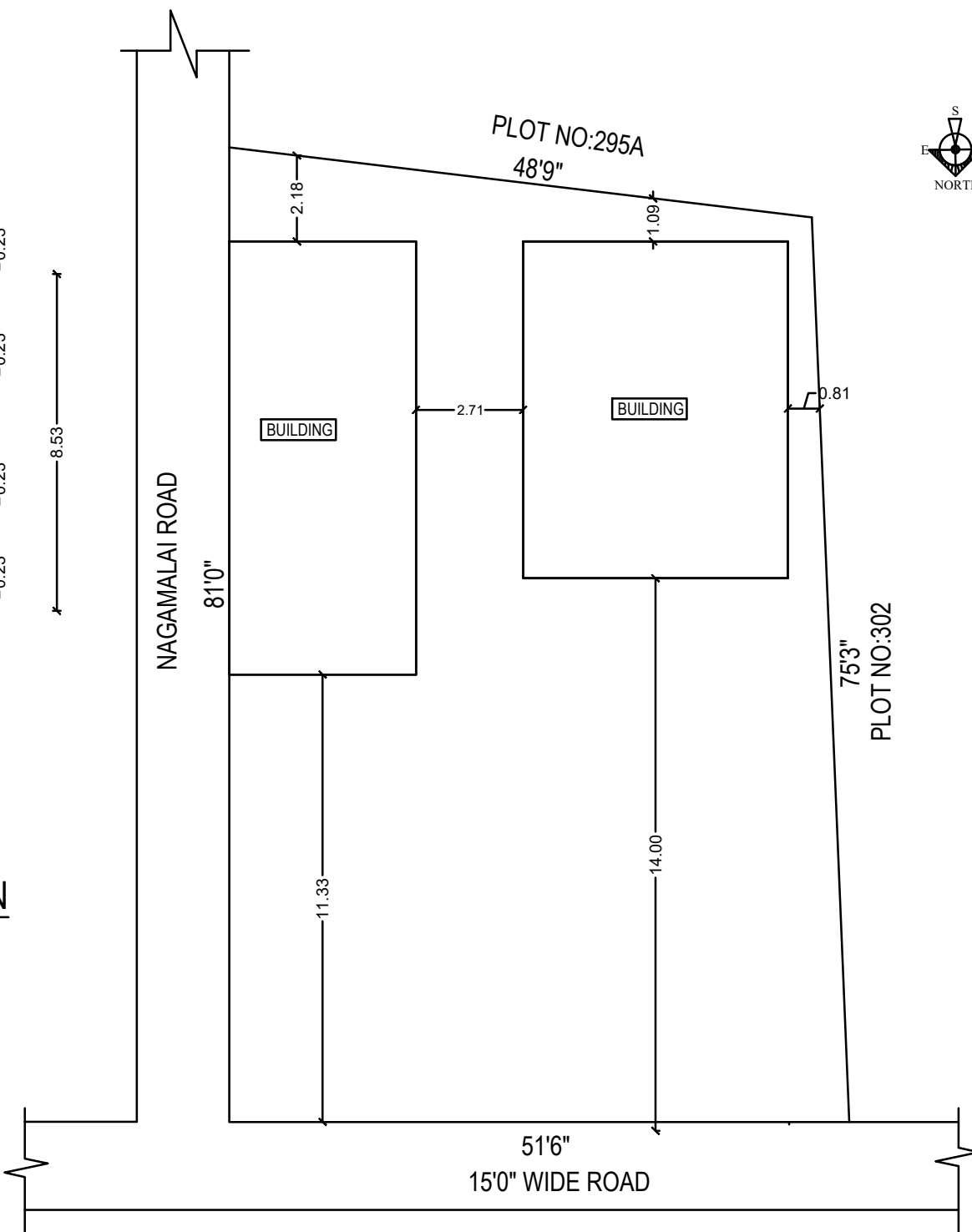
SITE PLAN
