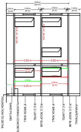
SECTION ON 'A-A'
