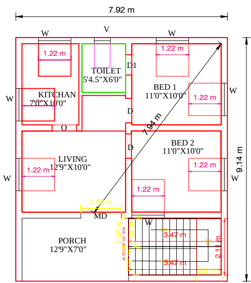
GROUND FLOOR PLAN [NORTH FACING]
