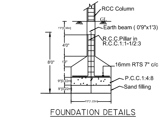
FOUNDATION DETAILS
