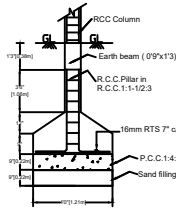
FOUNDATION DETAILS
