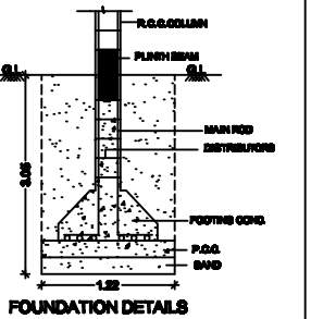
FOUNDATION DETAILS
