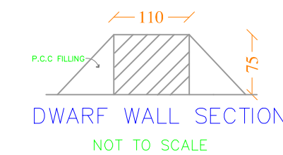
SECTION OF PEBBLE TRENCH SCALE : 1: = 100
