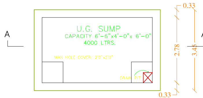
SUMP DETAIL SCALE 1"=4'-0"
