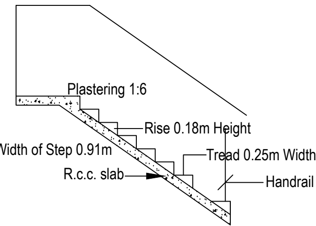
DETAILS OF STAIR CASE
