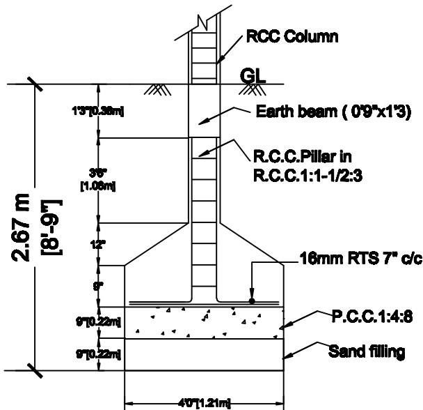
FOUNDATION DETAILS
