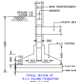
TYPICAL SECTION OF R.C.C COLUMN FOUNDATION
