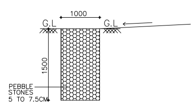
SECTION OF PEBBLE TRENCH SCALE : 1 : = 100
