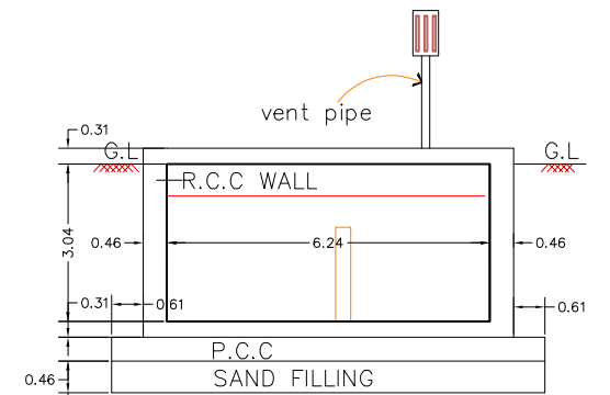
SECTION ON D-D
