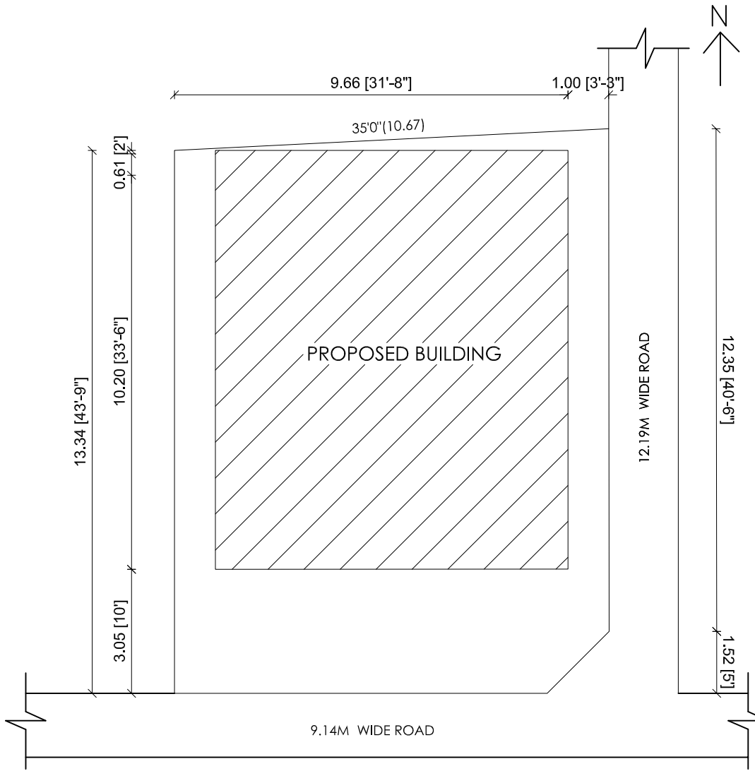
SITE PLAN
