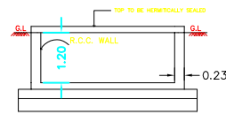
RWH SECTION (SAMPLE) RWH_CAPACITY_L = 2000LTRS
