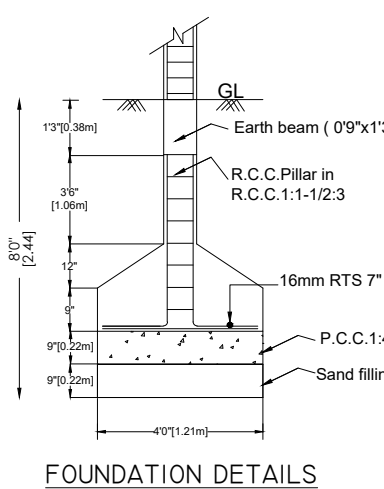
FOUNDATION DETAILS
