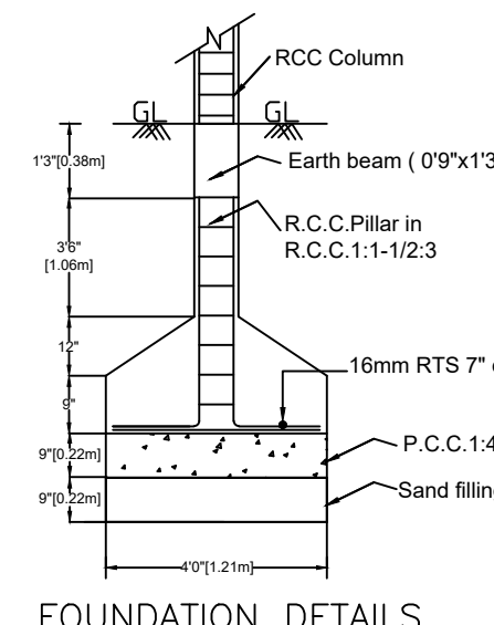
FOUNDATION DETAILS
