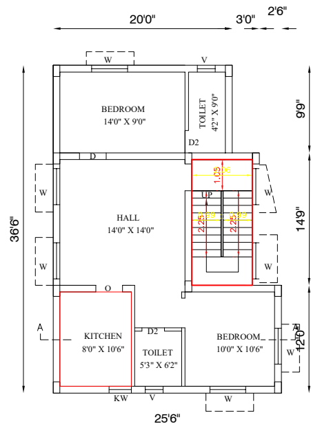
EXT.FIRST & SECOND FLOOR PLAN
