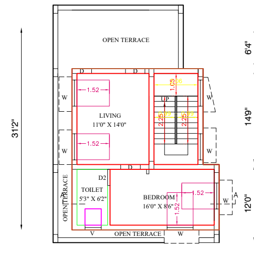
PRO.THIRD FLOOR PLAN
