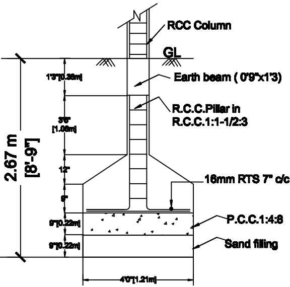
FOUNDATION DETAILS
