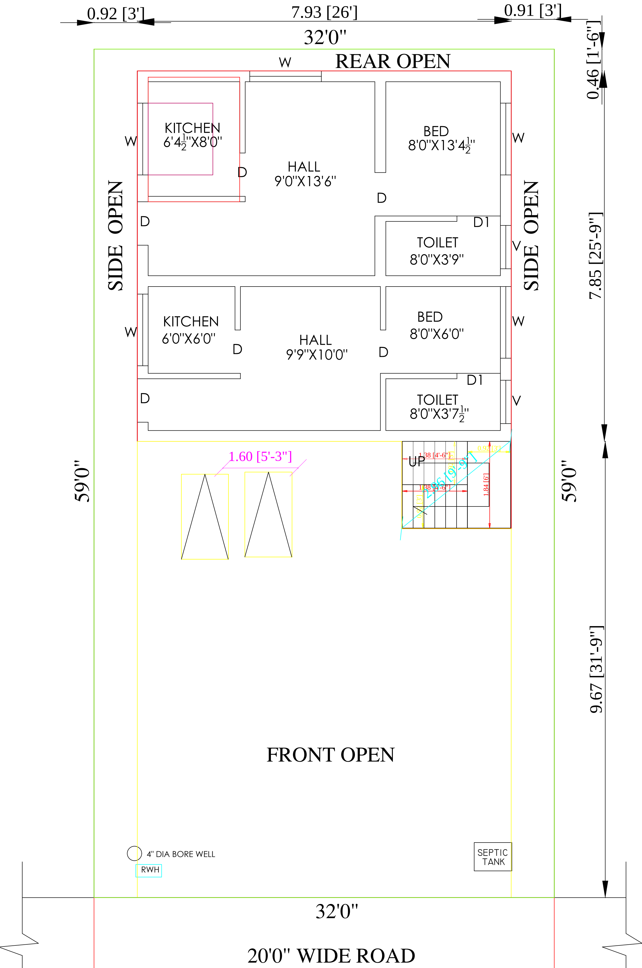
EXG & PRO .GROUND FLOOR PLAN
