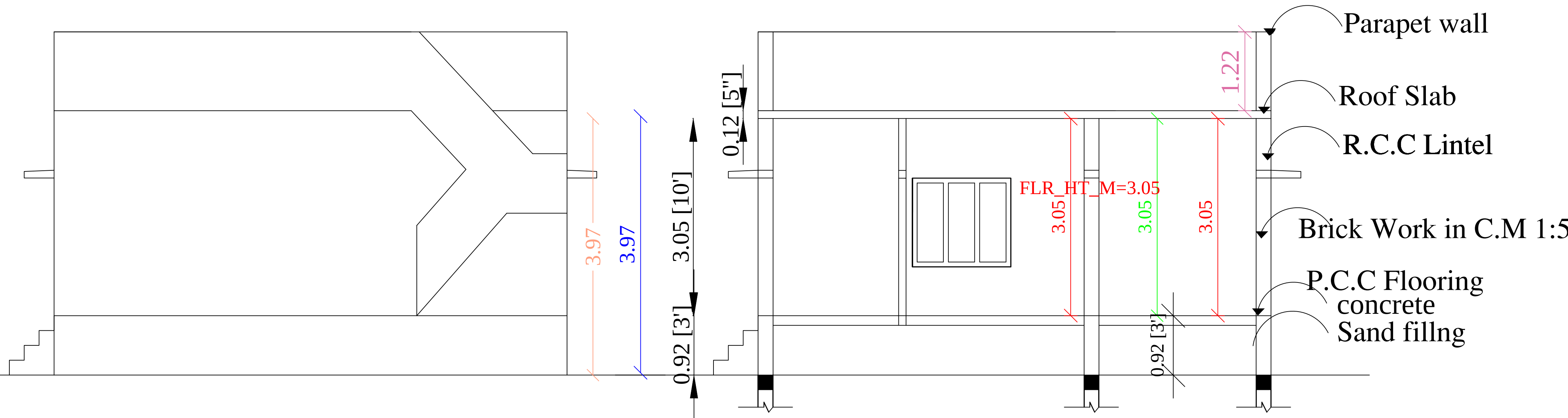
FRONT ELEVATION
