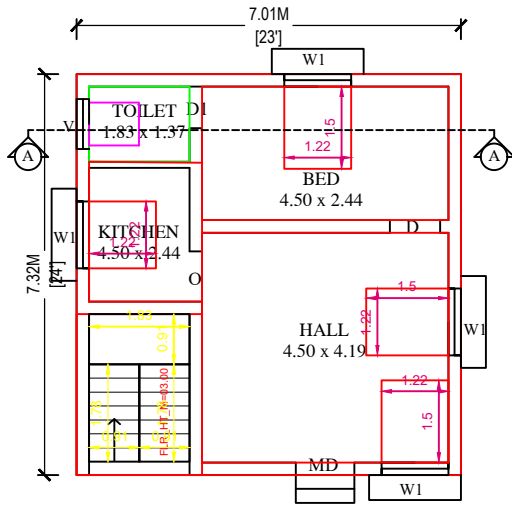
PRO.GOUND FLOOR PLAN
