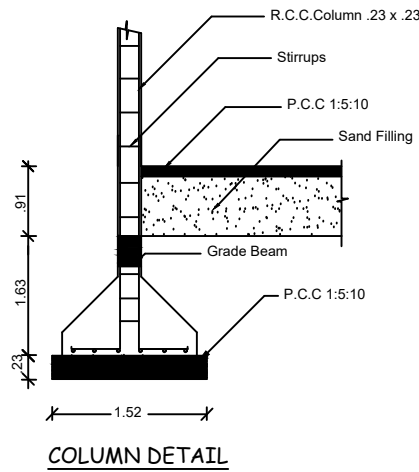
COLUMN DETAIL
