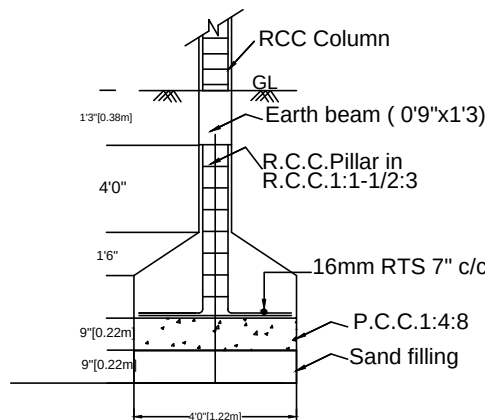
FOUNDATION DETAILS
