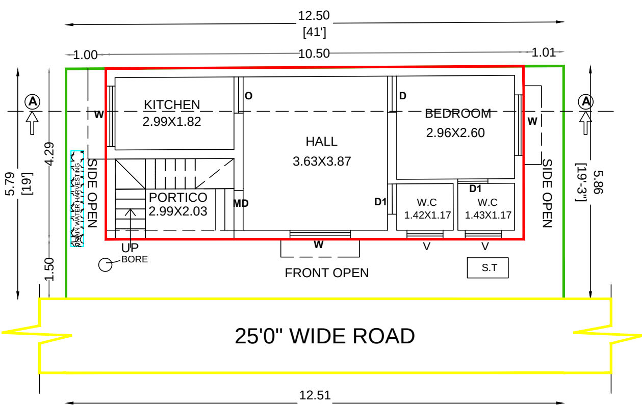
PRO.GROUND FLOOR PLAN
