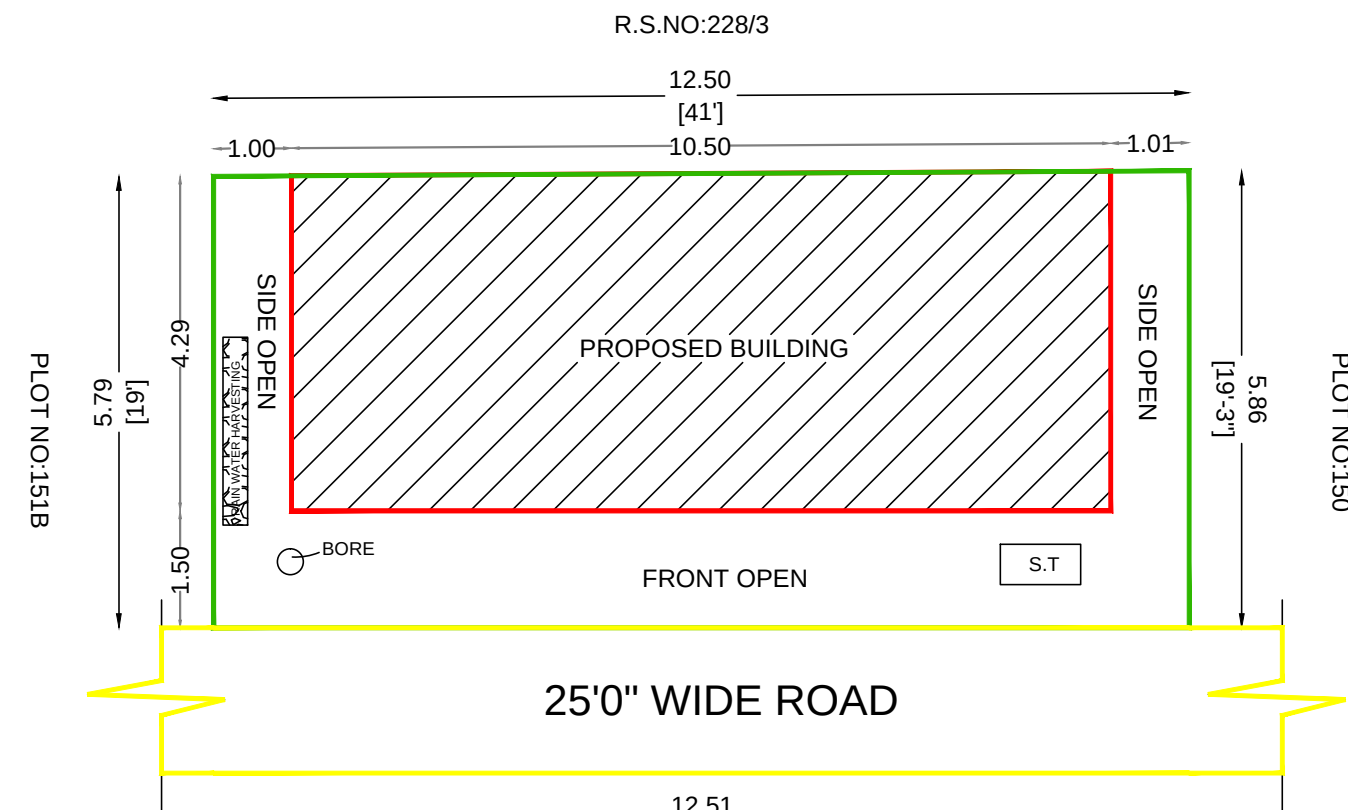
SITE PLAN
