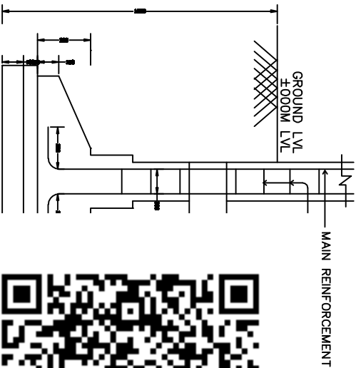
TYPICAL SECT R.C.C. COLUMN FC SCALE : 1" = 2'
