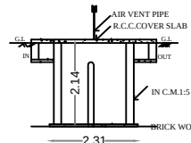
SEPTIC TANK DETAILS-SECTION
