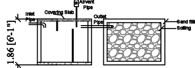
DETAILS OF SEPTIC TANK & DISPERSION TRENCH Details of solar water heating system
