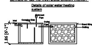
DETAILS OF SEPTIC TANK & DISPERSION TRENCH
