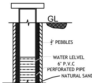
BORE WELL DETAILS
