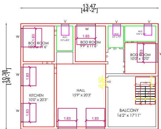
PRO.FIRST FLOOR PLAN
