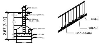
FOUNDATION DETAILS
