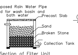
Section of Filter Unit
