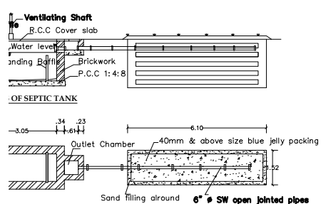
DETAILS OF SEPTIC TANK & DISPERSION TRENCH
